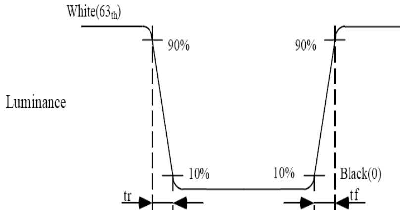
Fig.9-2: Definition of Response Time (White - Black)
