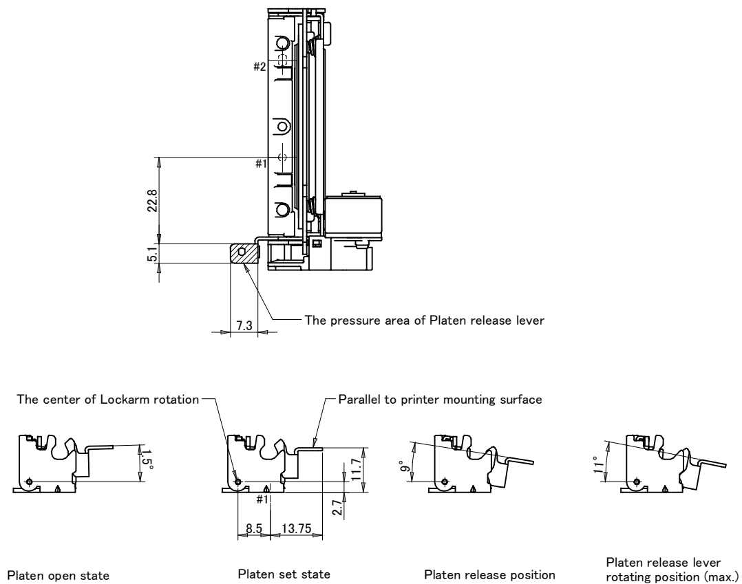
Figure 6-4 External Dimensions and Motion of the Platen Release Lever
