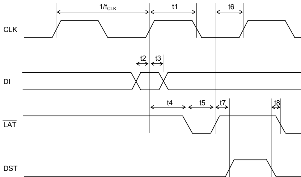
Figure 3-10 Thermal Head Drive Timing Chart
