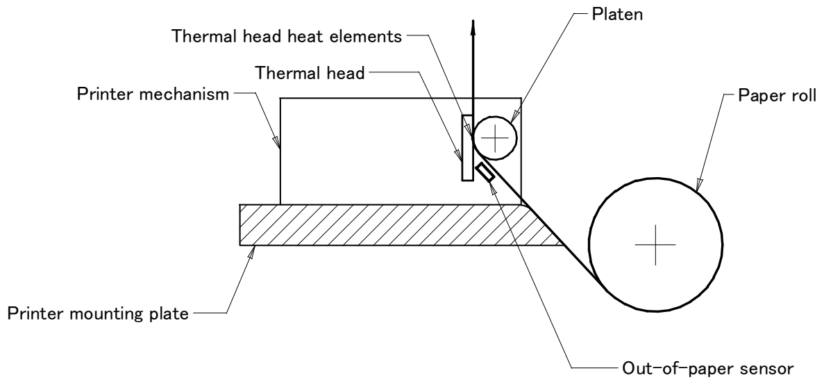
Figure 6-5 Recommended Layout between the Printer and the Thermal Paper
