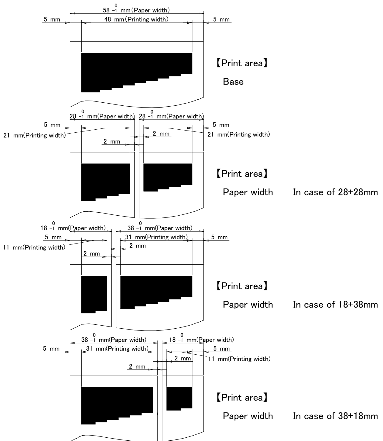
Figure 3-2 Print Area (LTPD245D)
