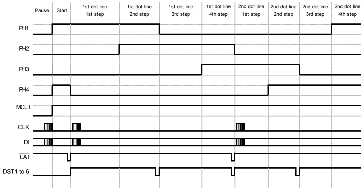
Figure 5-2 Timing Chart for Driving Using One Division (LTPD245D)
