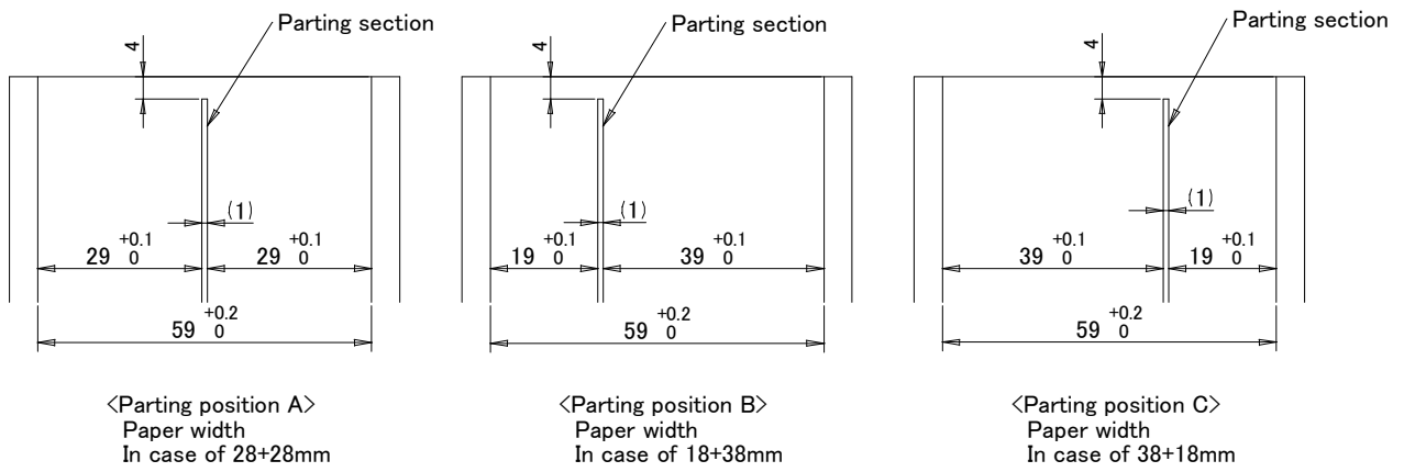
Figure 6-7 Recommended Separator (LTPD245D)
