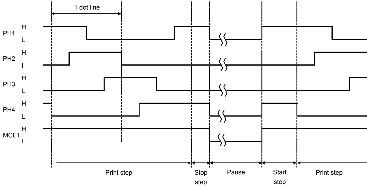
Figure 3-7 Motor Start/Stop Timing Chart
