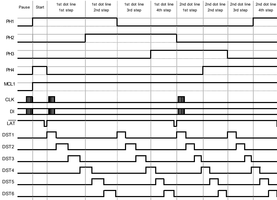
Figure 5-1 Timing Chart for Driving Using Six Divisions (LTPD245D)
