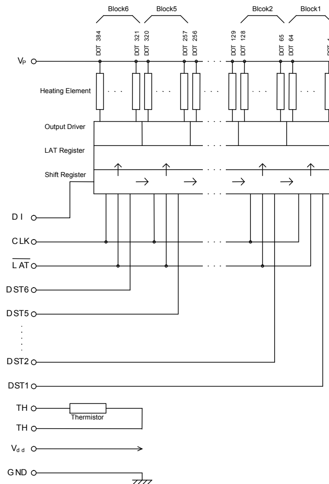
Figure 3-8 Thermal Head Block Diagram (LTPD245D)
