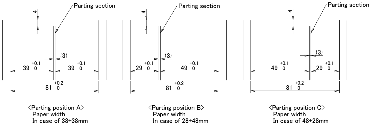
Figure 6-8 Recommended Separator (LTPD345D)
