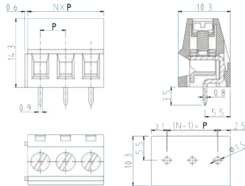
N: Number of poles P: Pitch
