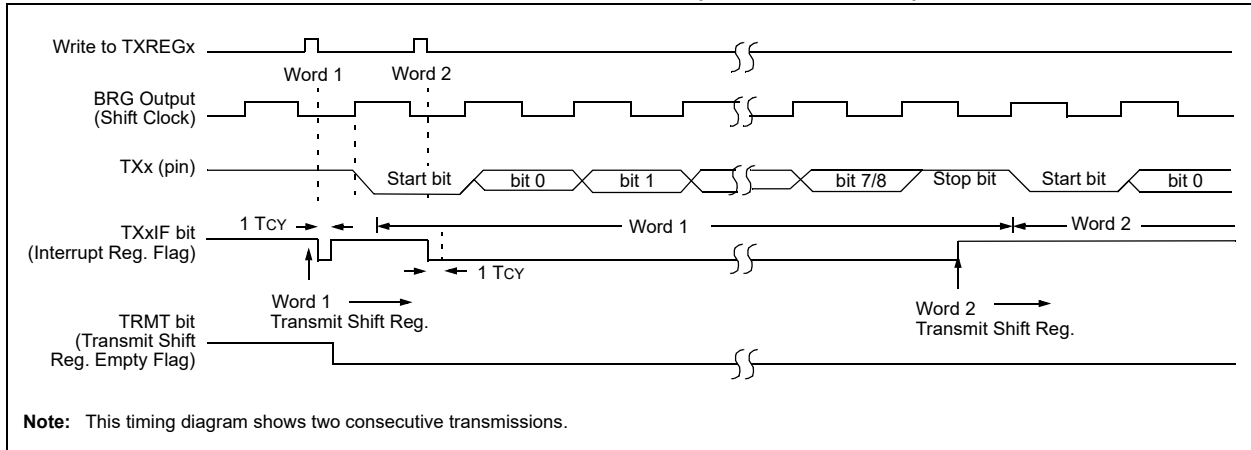
FIGURE 22-5: ASYNCHRONOUS TRANSMISSION (BACK-TO-BACK)
