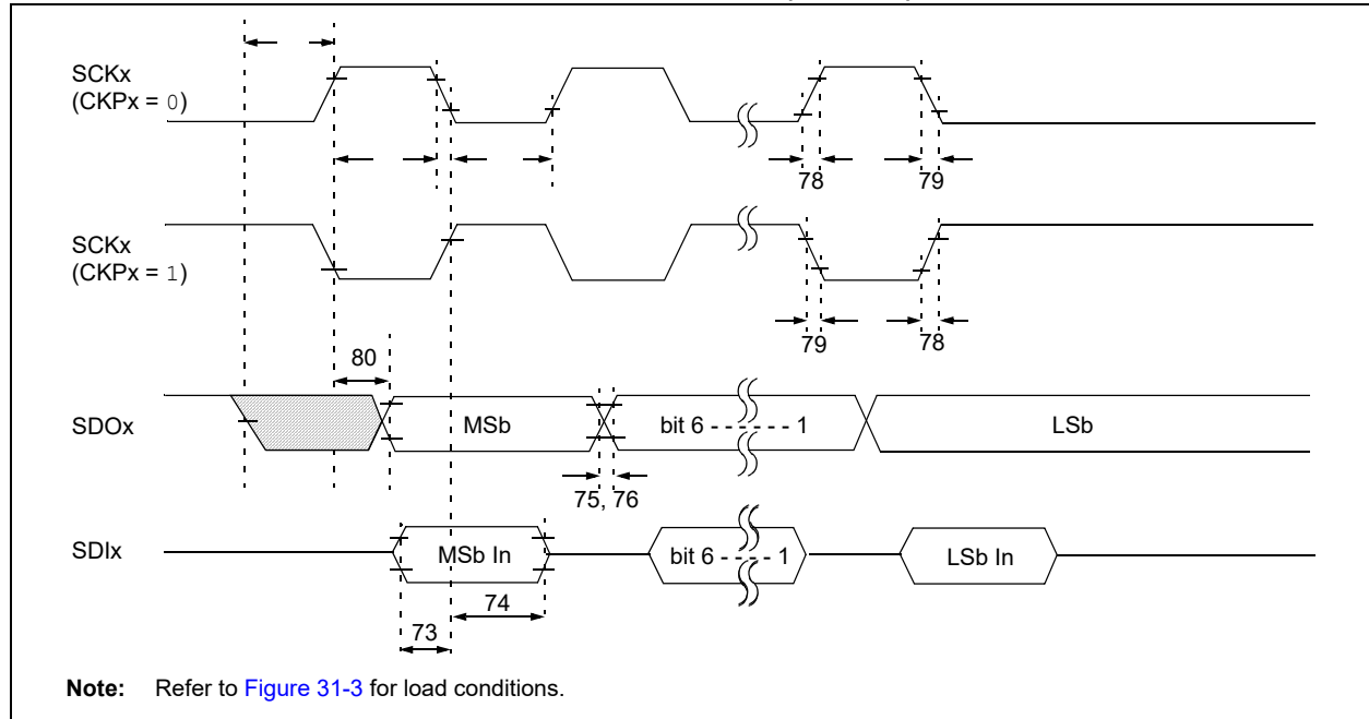
FIGURE 31-14: EXAMPLE SPI SLAVE MODE TIMING (CKE = 0)
