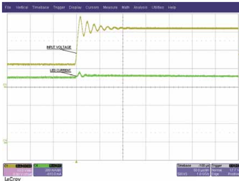
Fig. 5. Transient Response of LED Current to a Step Change in Input Current from 12V to 32V
