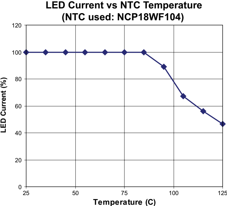
Fig. 10. Thermal Derating of the LED Current
