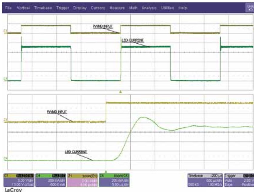
Fig. 3. PWM Dimming – Rising Edge Waveform
