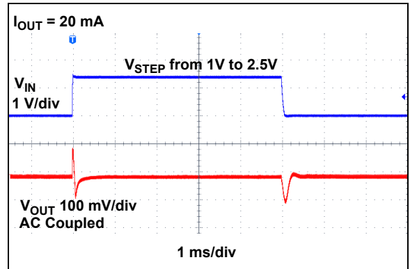
FIGURE 2-23: 3.3V V_{OUT} Line Transient Waveforms.
