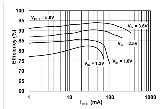
FIGURE 2-6: 5.0V V_{OUT} Efficiency vs. I_{OUT} .
