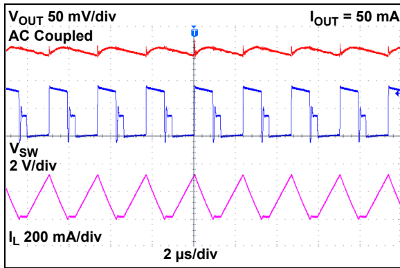
FIGURE 2-19: MCP16251 3.3V V_{OUT} PWM Mode Waveforms.
