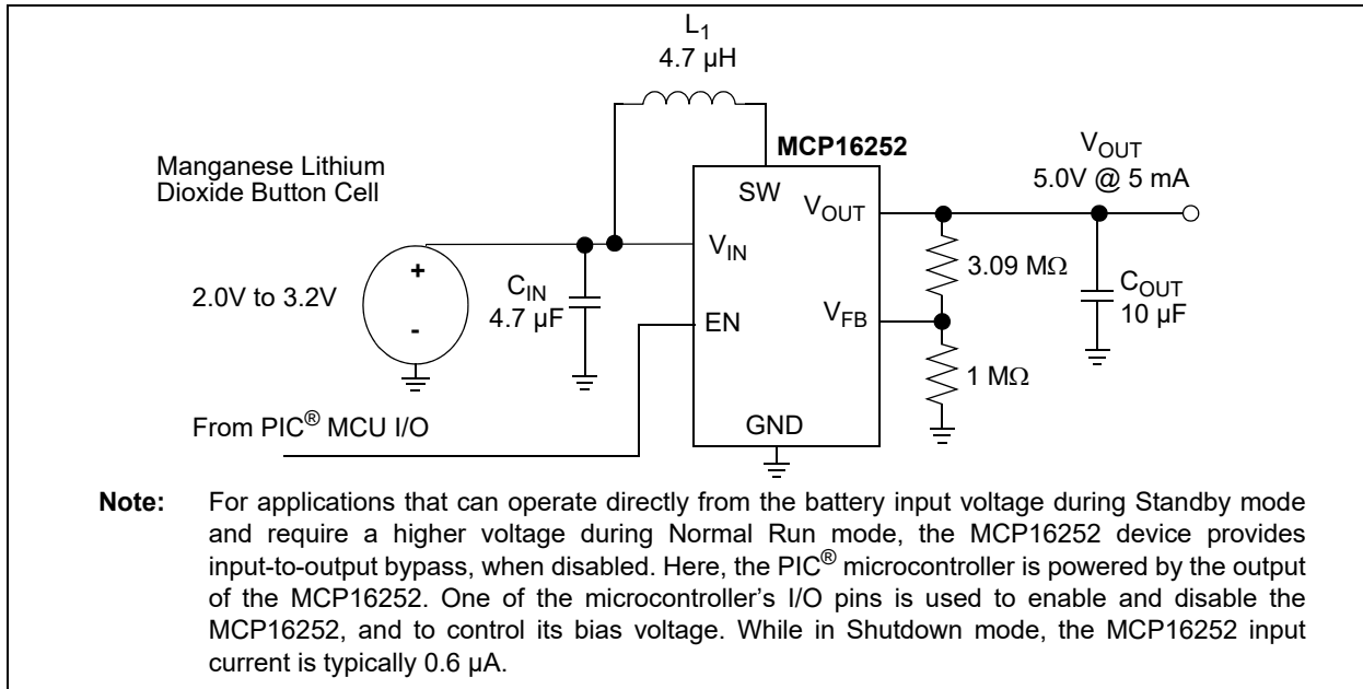
FIGURE 6-1: Manganese Lithium Coin Cell Application using I/O Bypass Mode.
