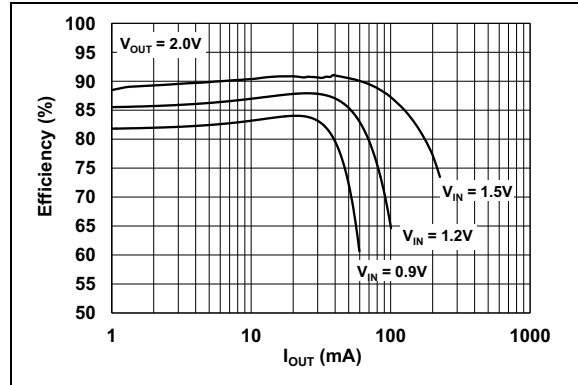
FIGURE 2-4: 2.0V V_{OUT} Efficiency vs. I_{OUT} .
