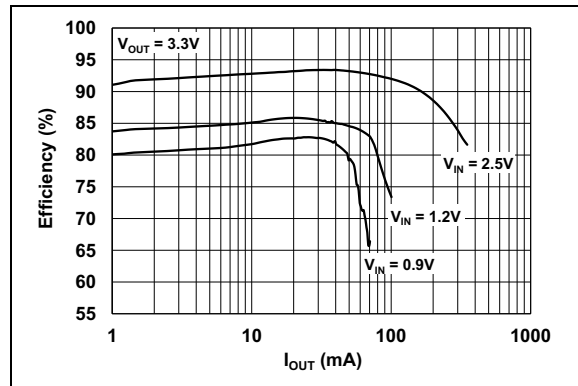
FIGURE 2-5: 3.3V V_{OUT} Efficiency vs. I_{OUT} .
