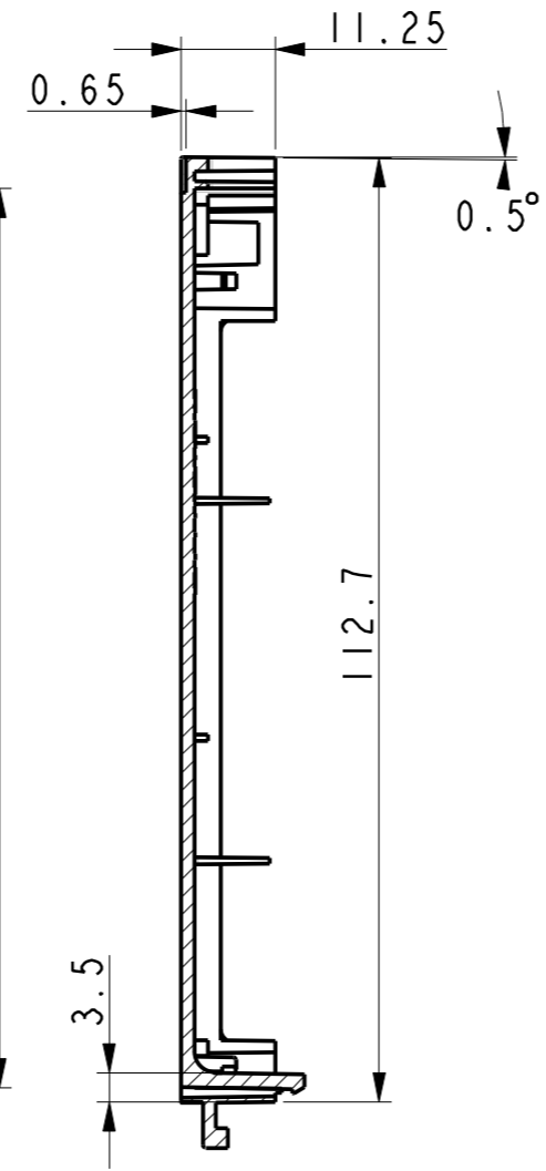
SECTION B-B
