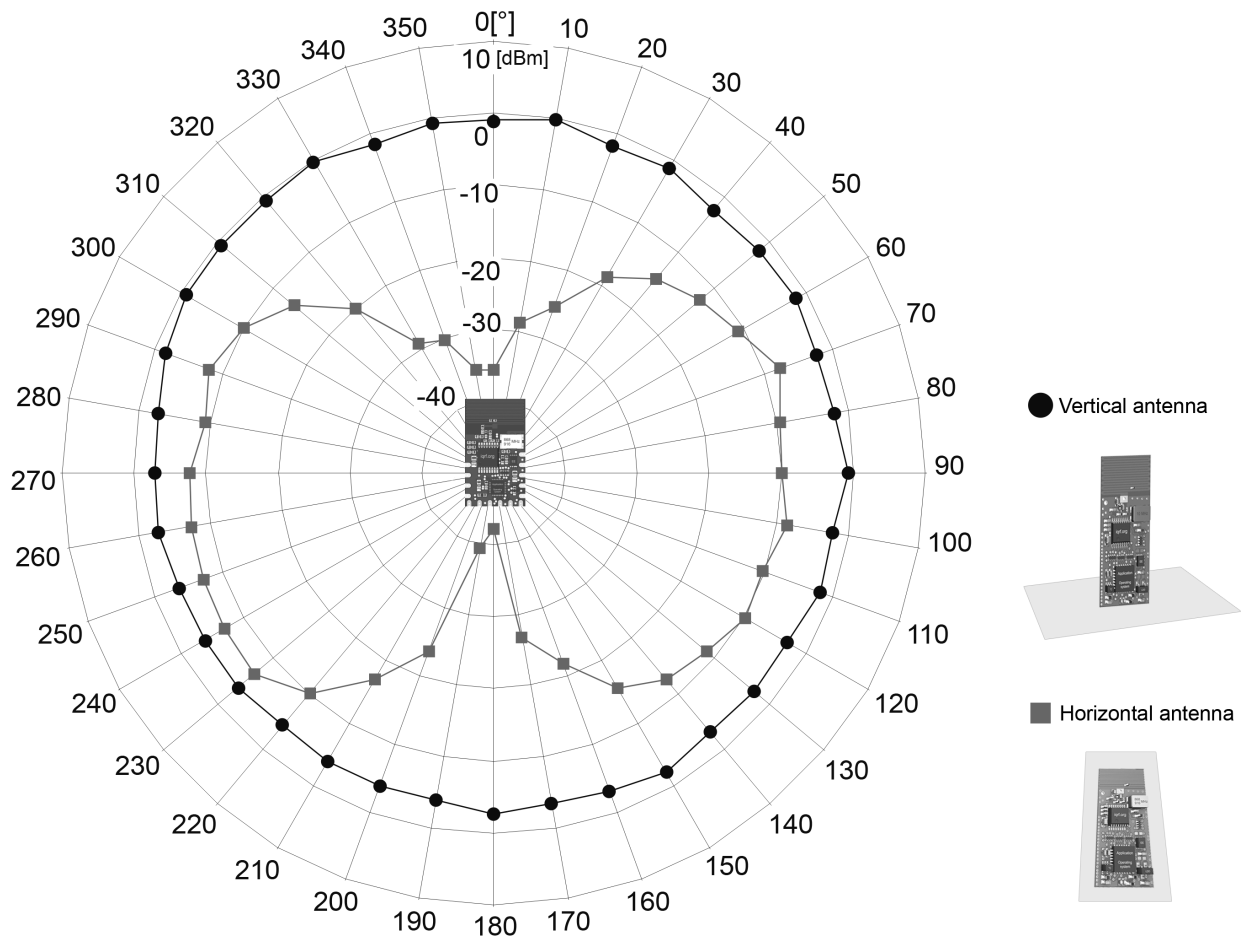
Figure 3: TR-52DA relative RF range vs. antenna orientation (radiation patterns)
