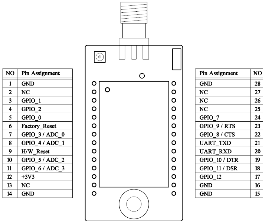
Figure 1-2 Pin Diagram
