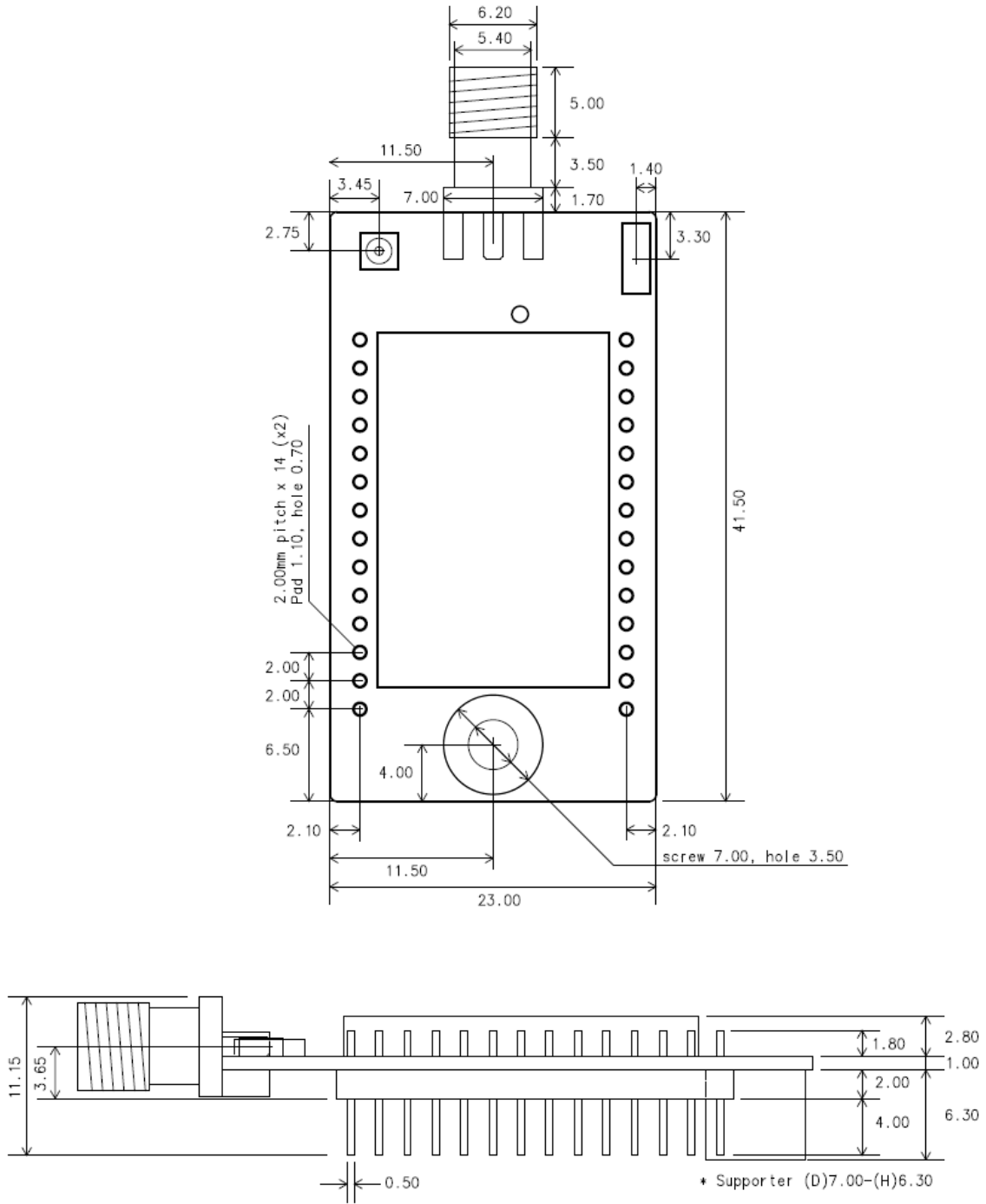
Figure 1-3 Mechanical Drawings
