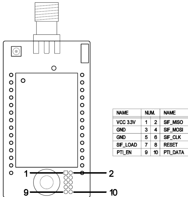
Figure 4-2 SIF Interface Pins
