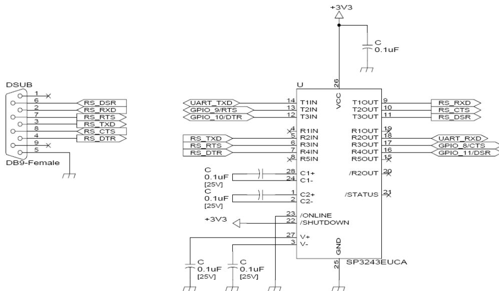
Figure 5-3 RS232 Serial
