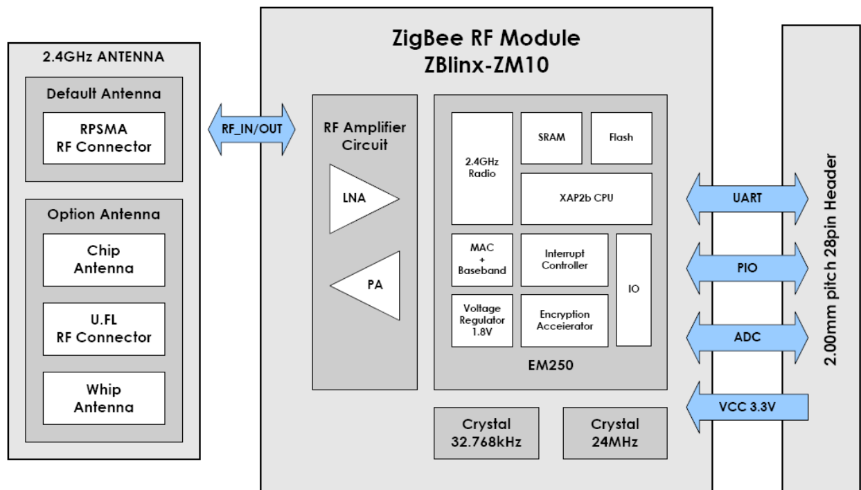
Figure 1-1 Device Diagram
