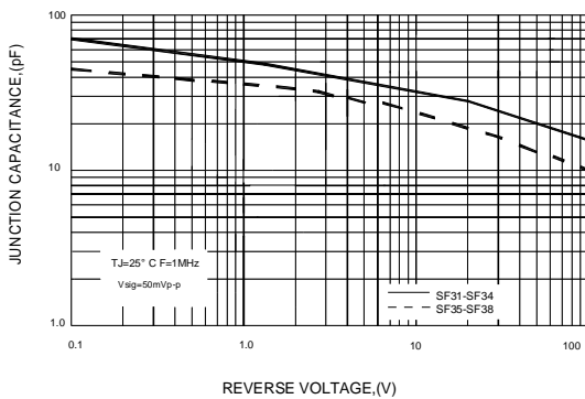
FIG.5-TYPICAL JUNCTION CAPACITANCE
