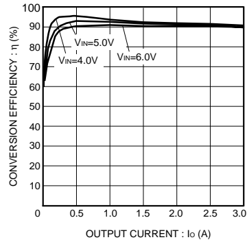
Fig.13 Conversion efficiency
