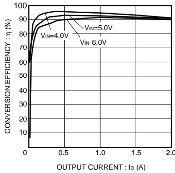
Fig.10 Conversion efficiency
