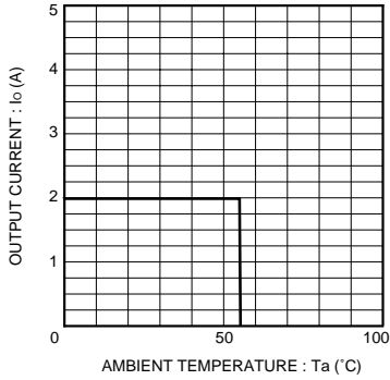
Fig.9 Derating curve
