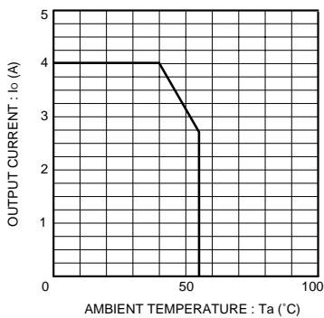
Fig.15 Derating curve
