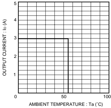
Fig.12 Derating curve
