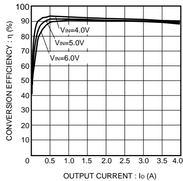
Fig.16 Conversion efficiency
