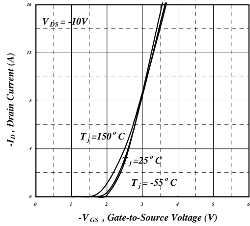
Fig 14. Transfer Characteristics
