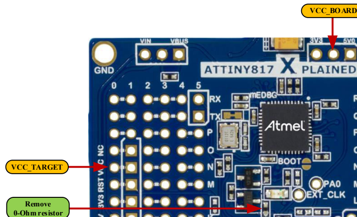
Figure 4-4. Current Measurement
