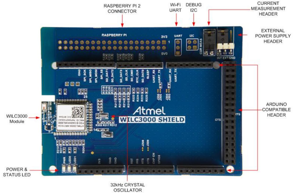
Figure 1-1. ATWILC3000 Shield Evaluation Kit Overview
