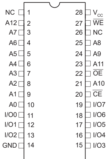
28-Lead PDIP/SOIC Top View
