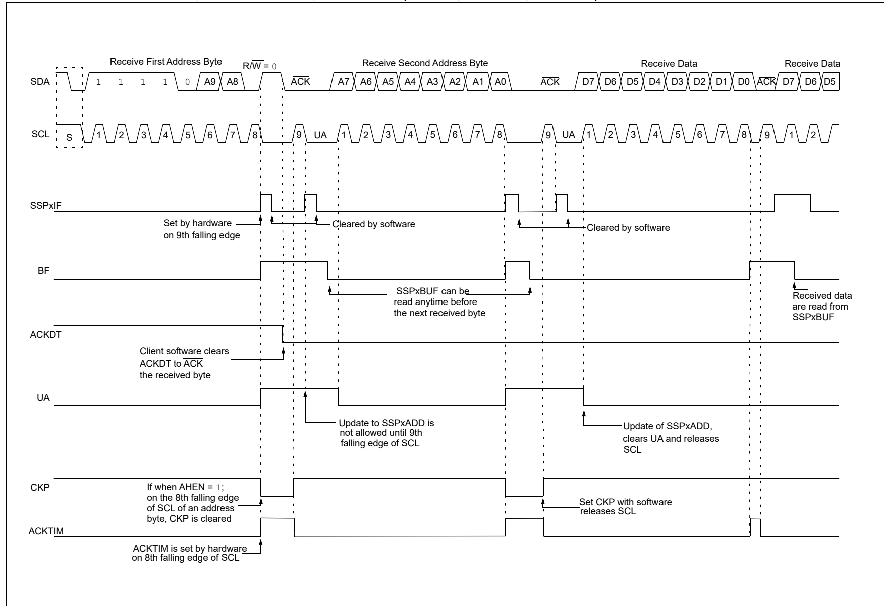
FIGURE 30-21: I 2 C CLIENT, 10-BIT ADDRESS, RECEPTION (SEN = 0, AHEN = 1, DHEN = 0)
