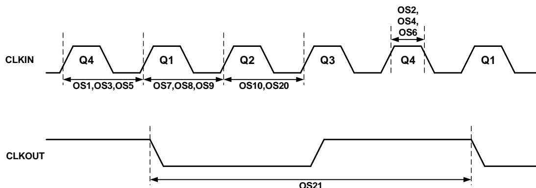
Figure 38-5. Clock Timing
