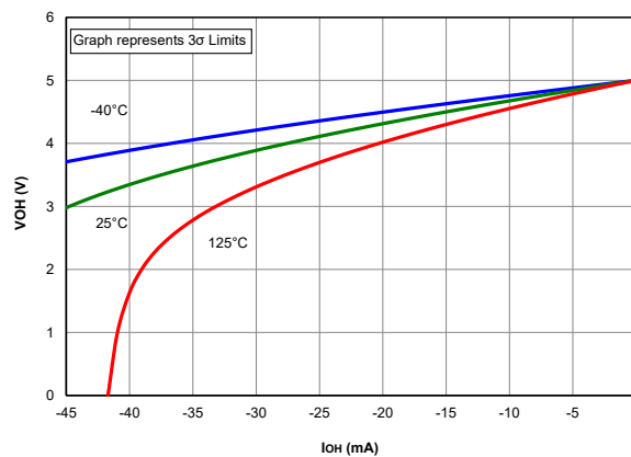
Figure 39-94. V_{OH} vs I_{OH} , Over Temperature, V_{DD} = 5.0V , PIC18F24/25K40 only
