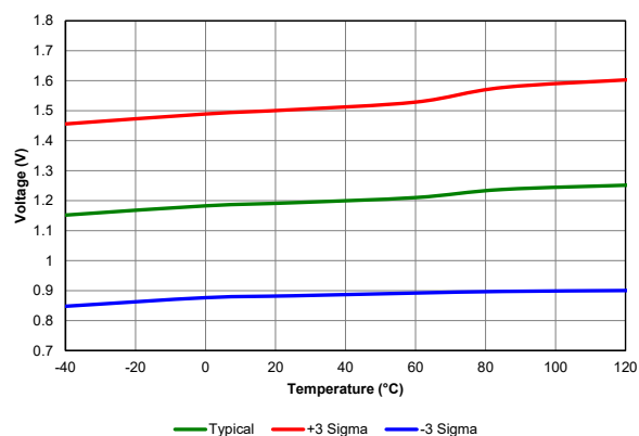
Figure 39-81. POR Rearm Voltage, VREGPM1 = 1, PIC18F24/25K40 only
