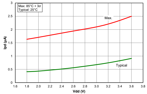
Figure 39-61. I_{PD} , Watchdog Timer, PIC18LF24/25K40 only
