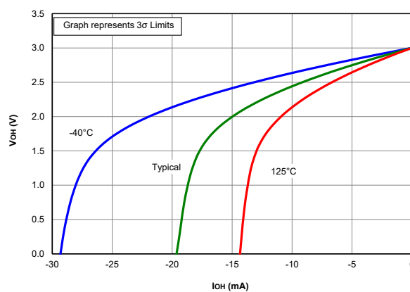
Figure 39-96. V_{OH} vs I_{OH} , Over Temperature, V_{DD} = 3.0V
