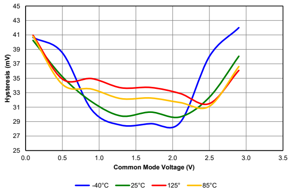
Figure 39-30. Comparator Hysteresis, V_{DD} = 3.0V , PIC18LF24/25K40 only
