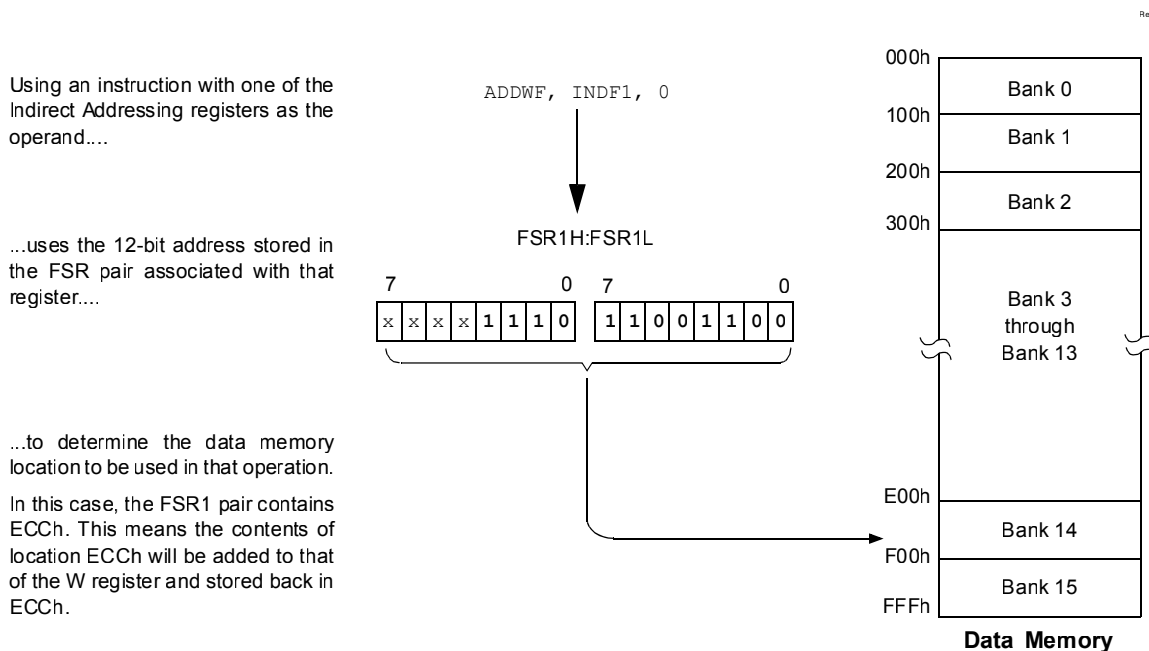
Figure 11-10. Indirect Addressing
