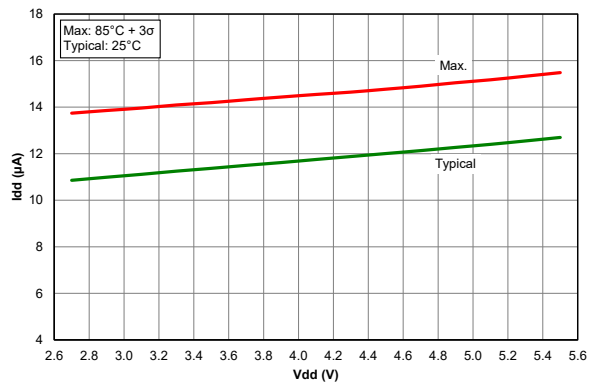
Figure 39-66. I_{PD} , Brown-out Reset, BORV = 1, PIC18F24/25K40 only
