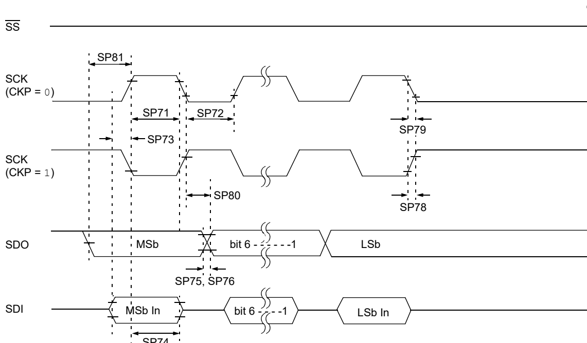
Figure 38-17. SPI Host Mode Timing (CKE = 1, SMP = 1)
