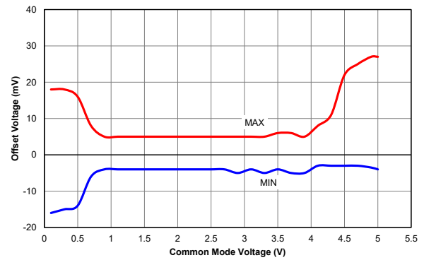
Figure 39-33. Comparator Offset, V_{DD} = 5.5V , from -40°C to 125°C, PIC18F24/25K40 only
