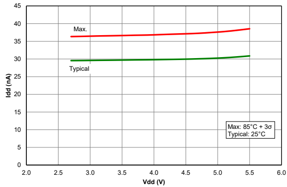
Figure 39-64. I_{PD} , Fixed Voltage Reference (FVR), PIC18F24/25K40 only
