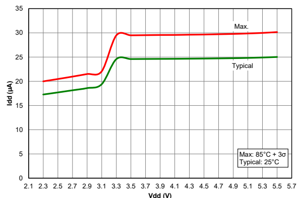
Figure 39-73. I_{PD} Base, VREGPM = 01, PIC18F24/25K40 only
