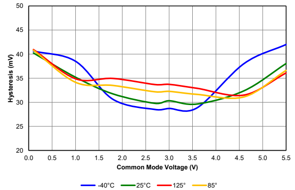
Figure 39-31. Comparator Hysteresis, V_{DD} = 5.5V , PIC18F24/25K40 only
