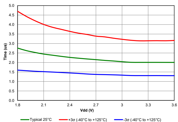
Figure 39-9. ADC RC Oscillator Period, PIC18LF24/25K40 only
