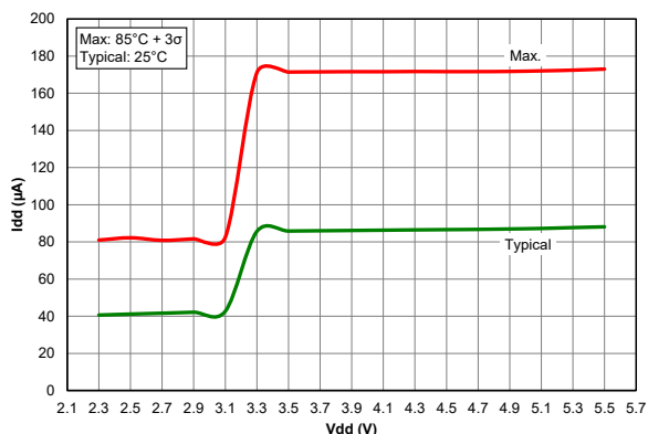
Figure 39-72. I_{PD} Base, VREGPM = 00, PIC18F24/25K40 only
