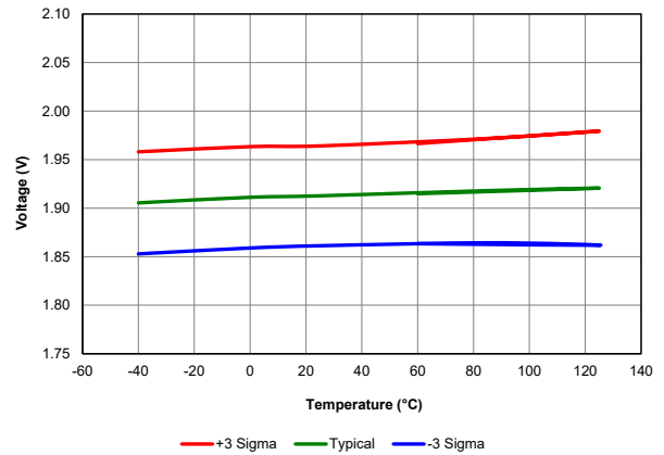
Figure 39-20. Brown-Out Reset Voltage, Trip Point (BORV = 11) for PIC18LF24/25K40 only
