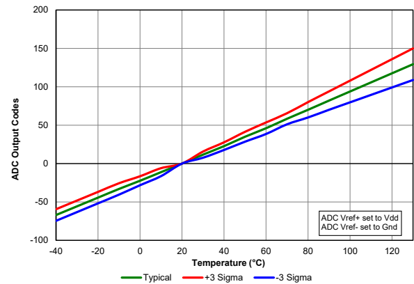
Figure 39-93. Temperature Indicator, Slope Normalized to 20°C, Low Range, V_{DD} = 2.3V , PIC18LF24/25K40 only
