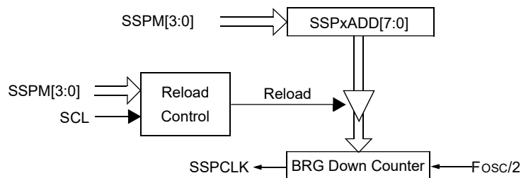
Figure 27-41. Baud Rate Generator Block Diagram
