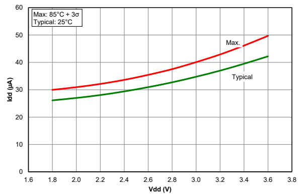
Figure 39-63. I_{DD} , Fixed Voltage Reference (FVR), PIC18LF24/25K40 only
