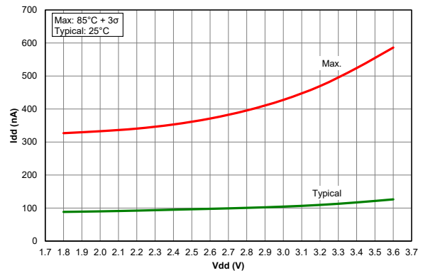
Figure 39-67. I_{PD} , Low-power Brown-out Reset, LPBOR = 0, PIC18LF24/25K40 only
