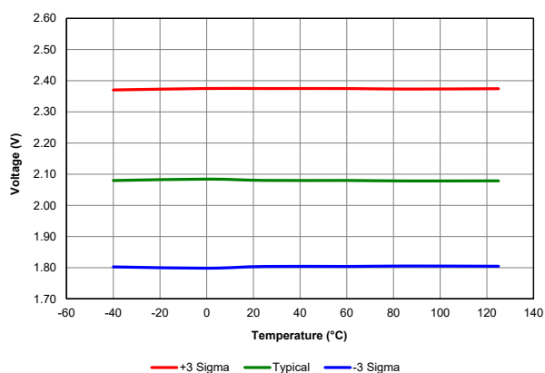
Figure 39-18. LPBOR Reset Voltage, PIC18LF24/25K40 only
