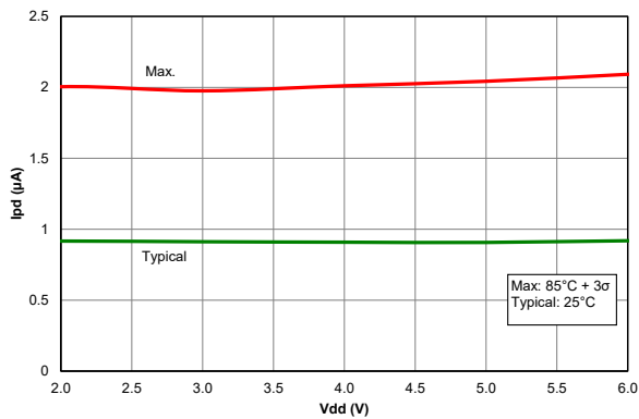
Figure 39-62. I_{PD} , Watchdog Timer, PIC18F24/25K40 only
