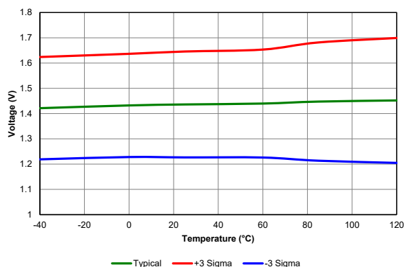
Figure 39-80. POR Rearm Voltage, VREGPM1 = 0, PIC18F24/25K40 only
