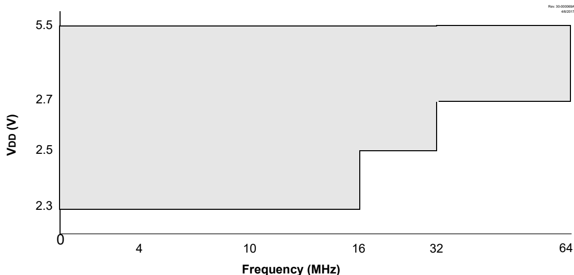
Figure 38-1. Voltage Frequency Graph, -40^{\circ}\text{C} \leq T_A \leq +125^{\circ}\text{C} , for PIC18F24/25K40 only
