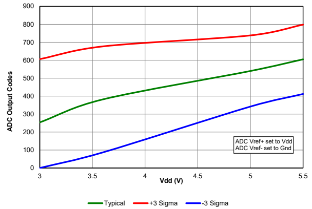
Figure 39-85. Temperature Indicator, Initial Offset, High Range, Temp = 20°C, PIC18F24/25K40 only
