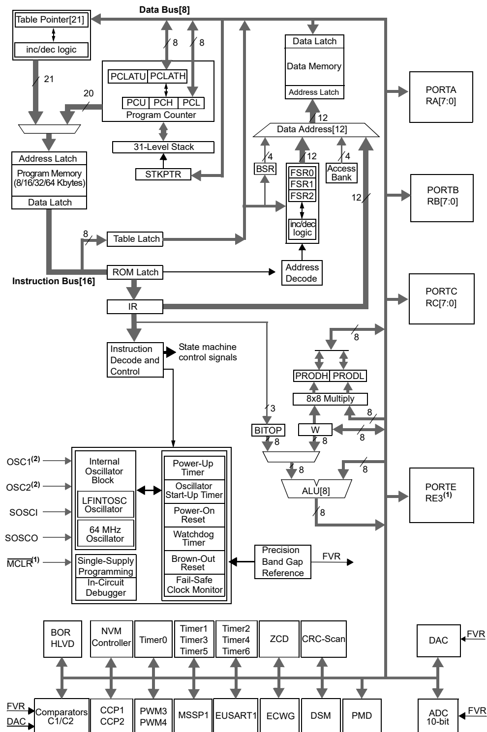
Figure 2-1. PIC18(L)F24/25K40 Family Block Diagram
