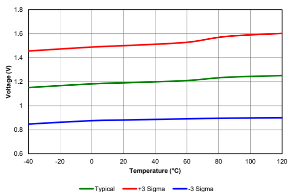
Figure 39-82. POR Rearm Voltage, Normal Power Mode, PIC18LF24/25K40 only
