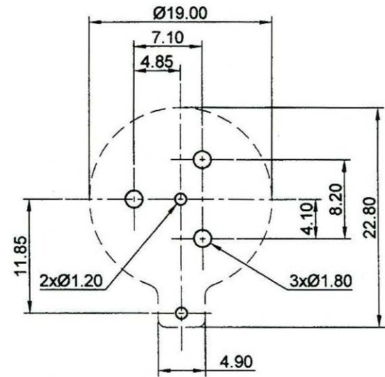
PCB MOUNTING LAYOUT
