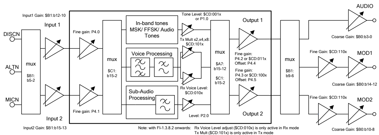
Figure 27 Level Adjustments
