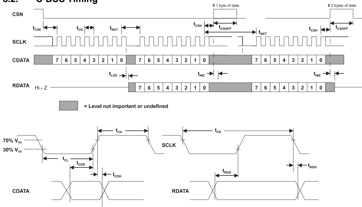
Figure 28 C-BUS Timing
