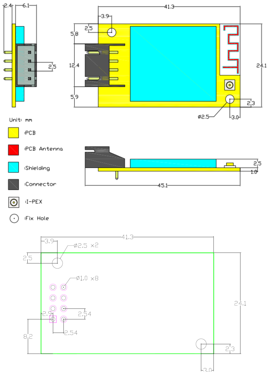
Figure 18. HF-LPB135 Mechanical Dimension
