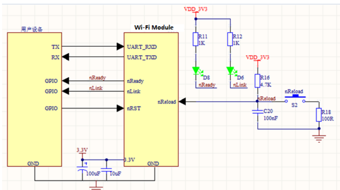
Figure 30. HF-LPX30 Hardware Typical Application
