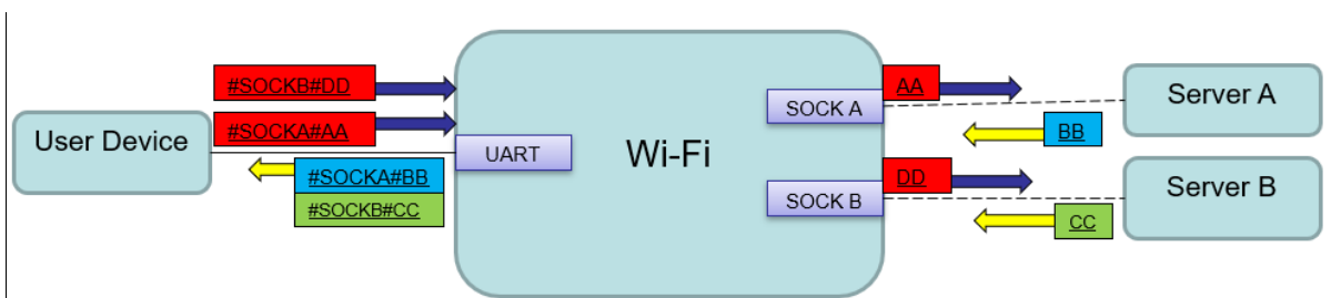
Figure 41. Two Socket Data Separation
