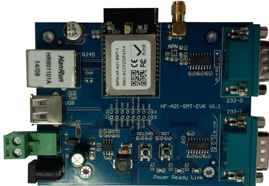
Figure 6. HF-A21-SMT Evaluation Kit
