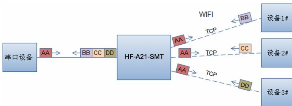
Figure 13. Multi-TCP Link Data Transmission Structure
