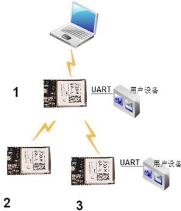
Figure 16. HF-A21-SMT AP Network Structure
