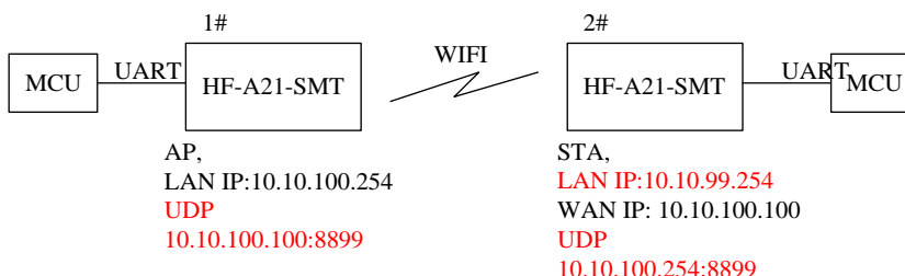
Figure 45. Configure Transparent Serial Port Connection (UDP)
