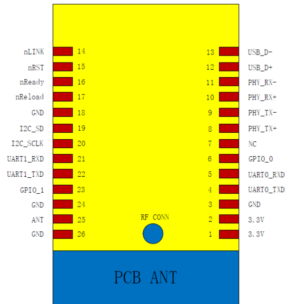
Figure 2. HF-A21-SMT Pins Map
