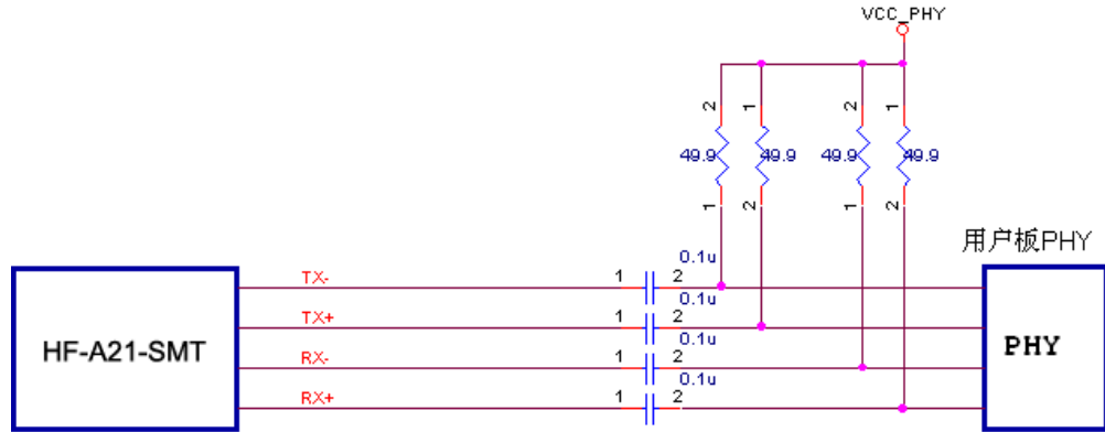
Figure 10. Ethernet Reference Design without Transformer
