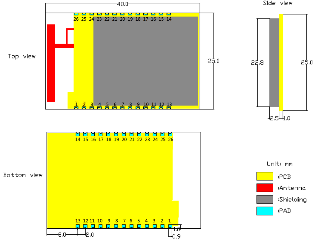
Figure 3. HF-A21-SMT Mechanical Dimension
