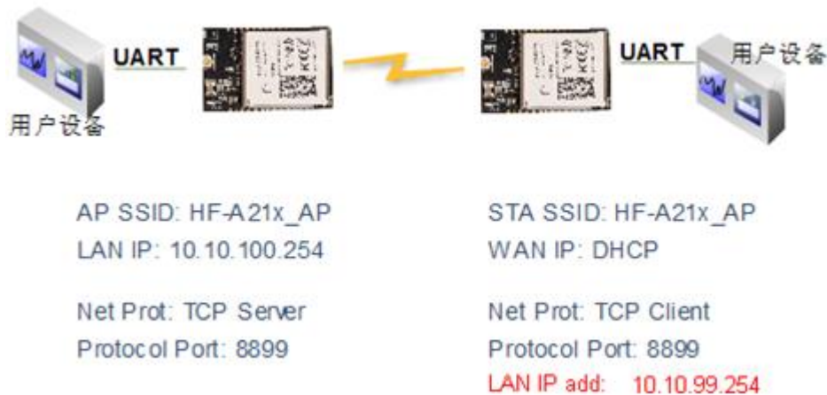
Figure 36. Transparent Serial Port Application
