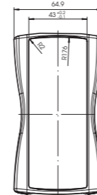
Base - external view
