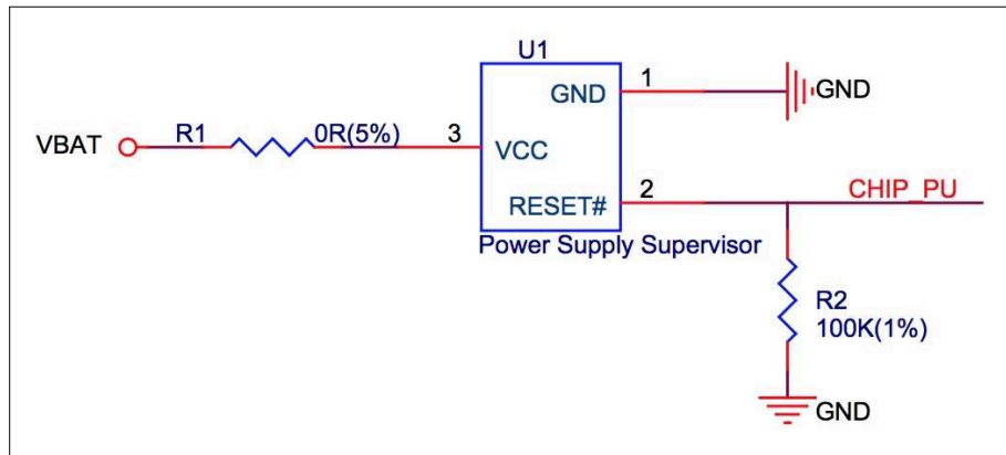
Figure 6: Reset Circuit
