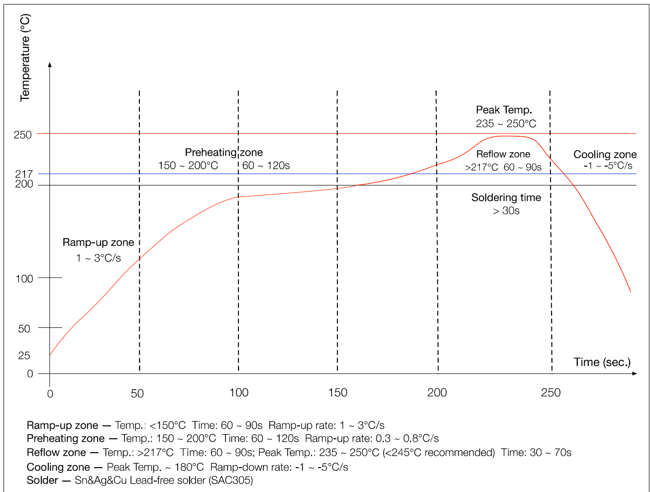
Figure 2: Reflow Profile
