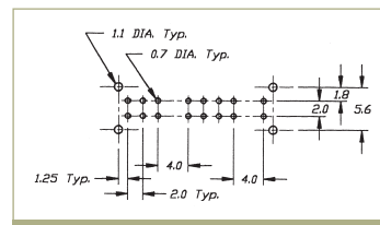
P.C. MOUNTING
