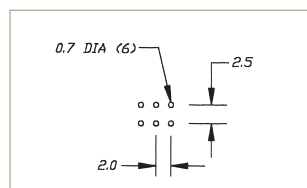
P.C. MOUNTING
