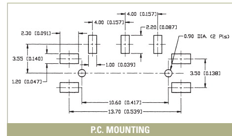
P.C. MOUNTING
