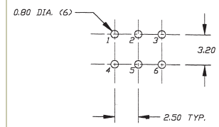
P.C. MOUNTING
