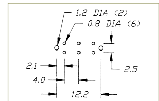
P.C. MOUNTING
