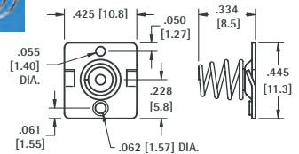
DUAL CONTACTS
