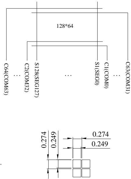
SCALE 10/1
