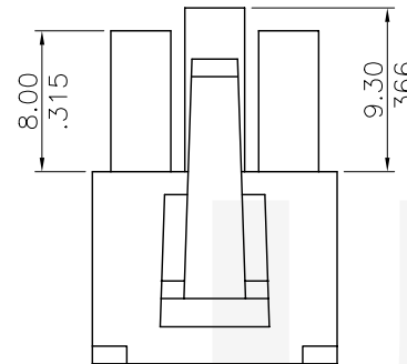
FOR 3 CIRCUITS
