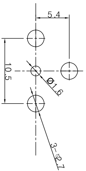
PCB Layout ( \pm 0.1 )
