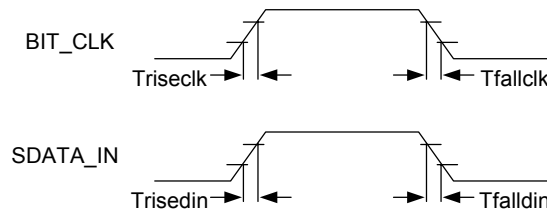
Signal Rise and Fall timing diagram
