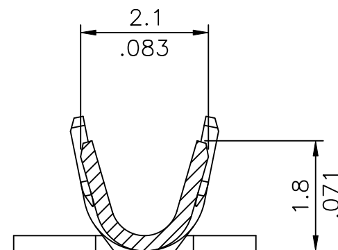
SEC. X-X
