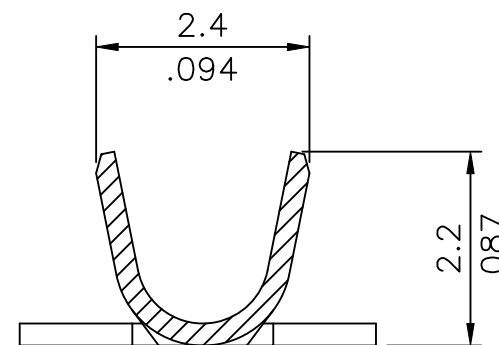
SEC. Y-Y
