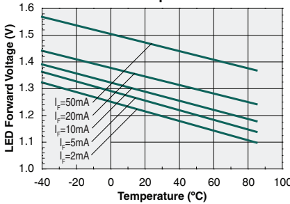
LED Forward Voltage vs. Temperature
