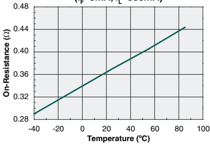
Typical On-Resistance vs. Temperature DC-Only Configuration ( I_F=0mA, I_L=1A )
