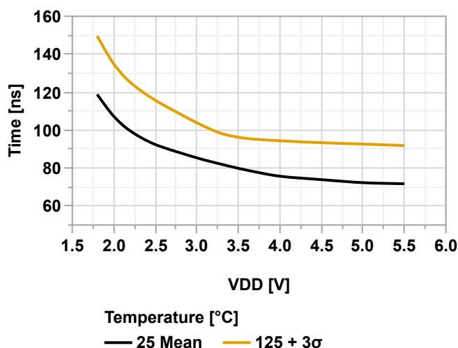
Figure 40-131. Falling Edge Response Time vs. V_{DD} ( V_{CM} = V_{DD}/2 , CTRLA.POWER = 0x01)
