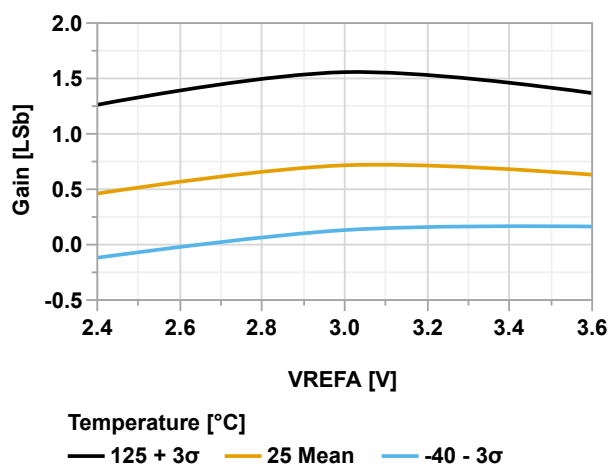
Figure 40-116. Negative Gain Error vs. V_{\text{REFA}} (ADC Differential Mode @60 kps, V_{\text{DD}} = 3.6\text{V} )
