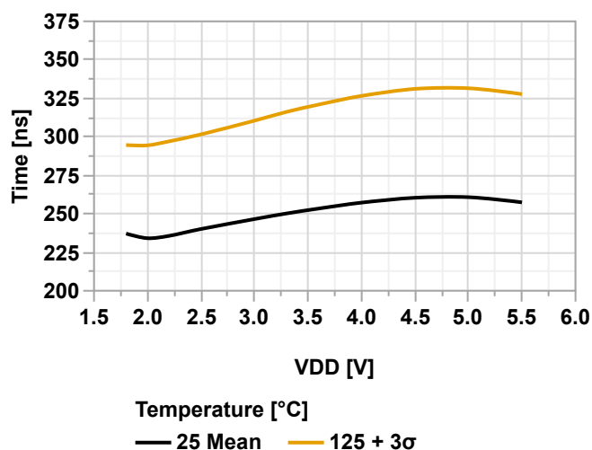
Figure 40-132. Rising Edge Response Time vs. V_{DD} ( V_{CM} = V_{DD}/2 , CTRLA.POWER = 0x01)
