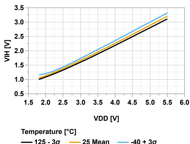
Figure 40-70. Input Pin with I 2 C Trigger - Minimum V_{IH} vs. V_{DD}
