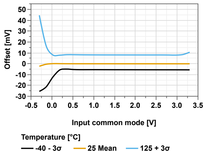
Figure 40-176. Offset Over V_{CM} and Temperature
