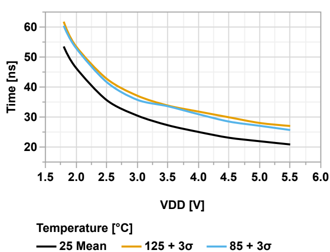
Figure 40-63. Fall Time vs. V_{DD} (PORTCTRL.SRL = 0x01)
