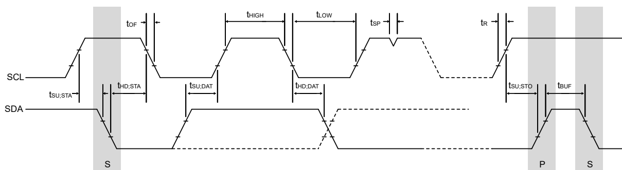
Figure 39-7. TWI - Timing Requirements
