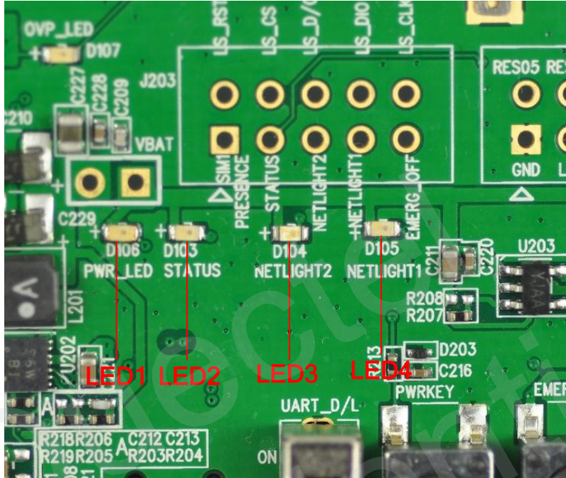
Figure 47: Operating status LED
