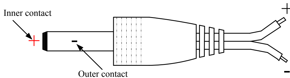
Figure 7: Power plug
