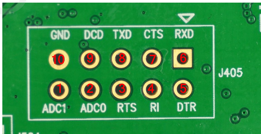
Figure 52: CON2
