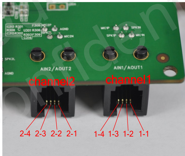
Figure 13: Audio interface
