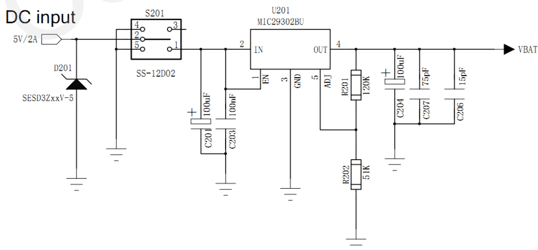
Figure 5: Reference circuit of the power supply
