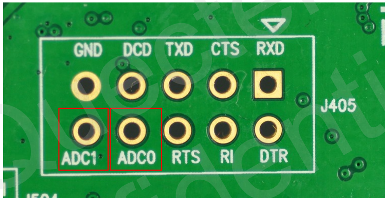
Figure 49: Test point of ADC
