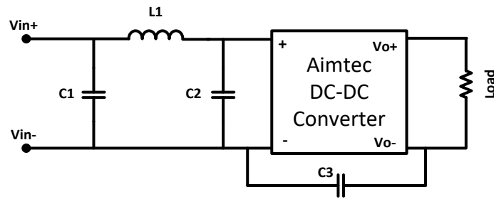
EMI Filtering circuit
