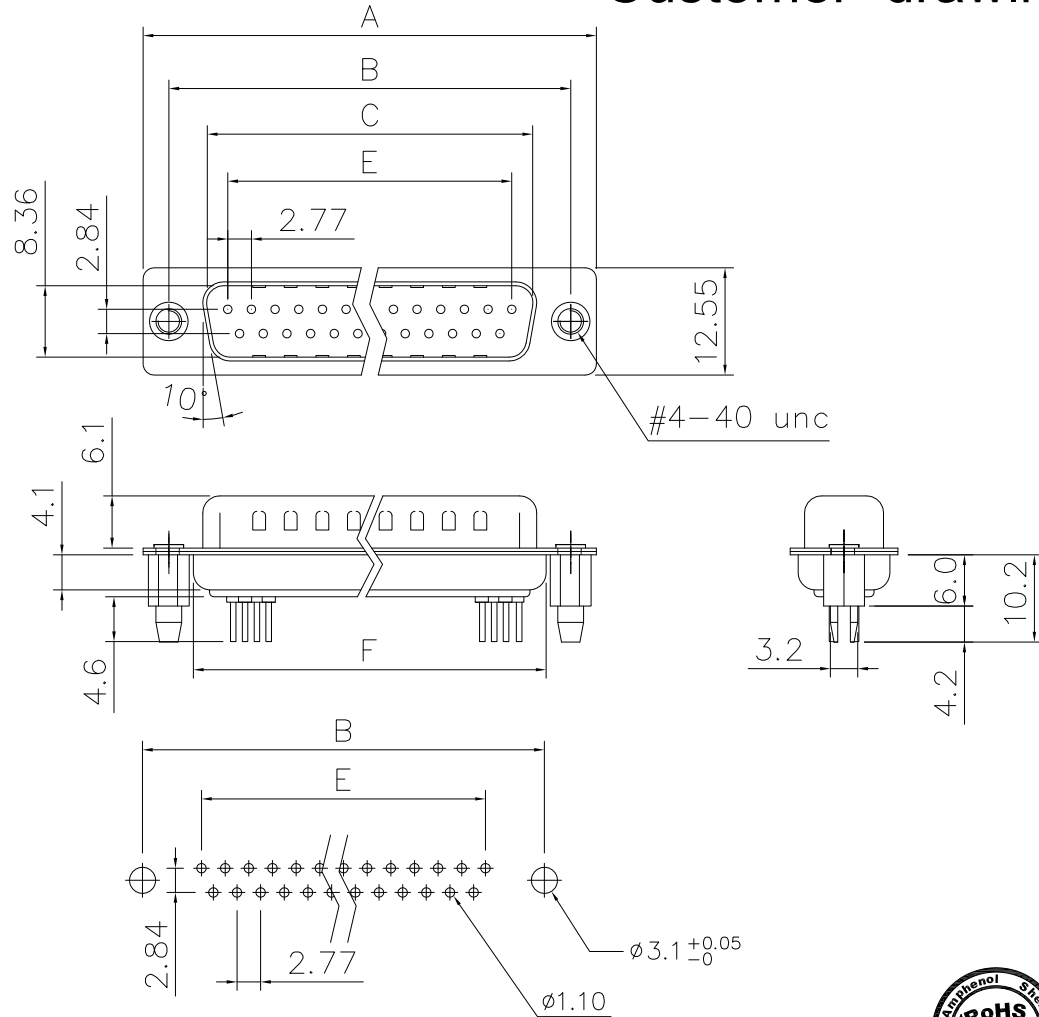
RECOMMENDED P.C.B LAYOUT (TOLERANCE +/-0.05)
