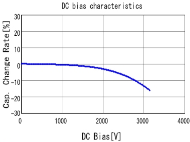
■ GRM42A7U3F101JW31 C-DC bias capchange, 25.0degC, AC1V
