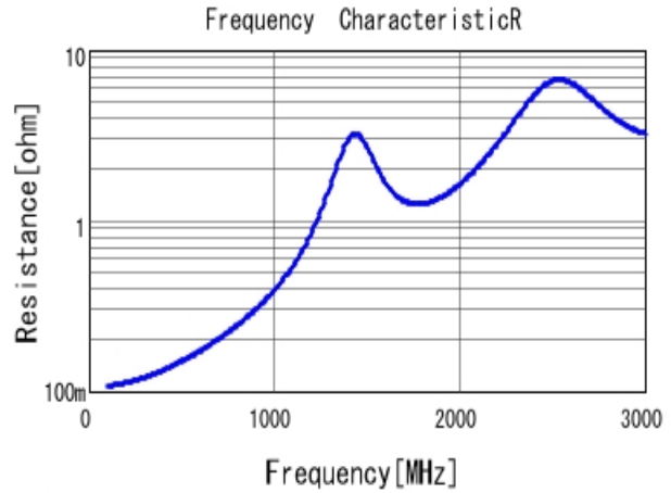
■ GRM42A7U3F101JW31 R DCOV, 25degC
