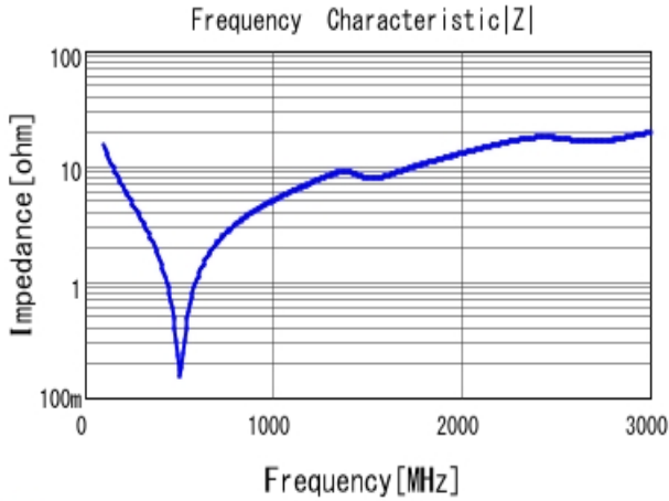
■ GRM42A7U3F101JW31 |Z| DCOV, 25degC
