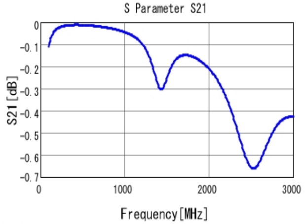
■ GRM42A7U3F101JW31 S21 DCOV, 25degC
