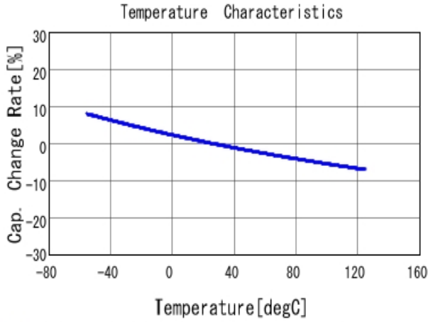
■ GRM42A7U3F101JW31 C-Temp. capchange, DCOV, AC1Vrms
