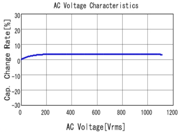
■ GRM42A7U3F101JW31 C-AC Voltage capchange, DCOV, 25.0d
