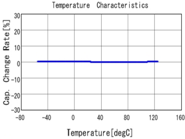
■ GRM1885C1H103JA01 C-Temp. capchange, DCOV, AC1Vrms
