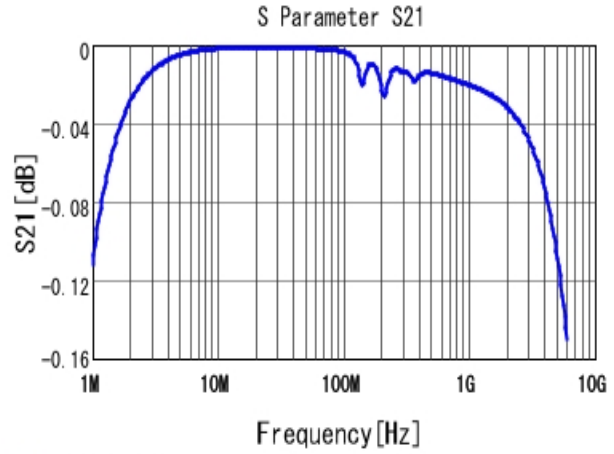
■ GRM1885C1H103JA01 S21 DCOV, 25degC
