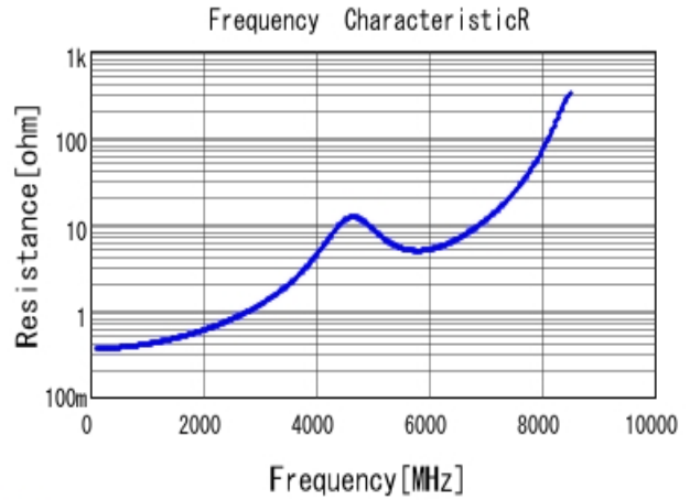
■ GRM1885C1H120JA01 R DCOV, 25degC
