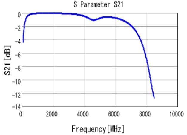
■ GRM1885C1H120JA01 S21 DCOV, 25degC
