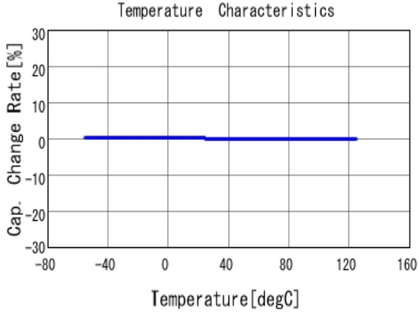
■ GRM1885C1H120JA01 C-Temp. capchange, DCOV, AC1Vrms
