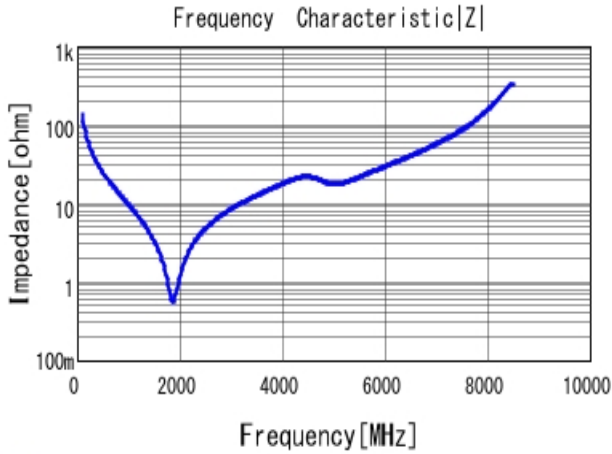
■ GRM1885C1H120JA01 |Z| DCOV, 25degC
