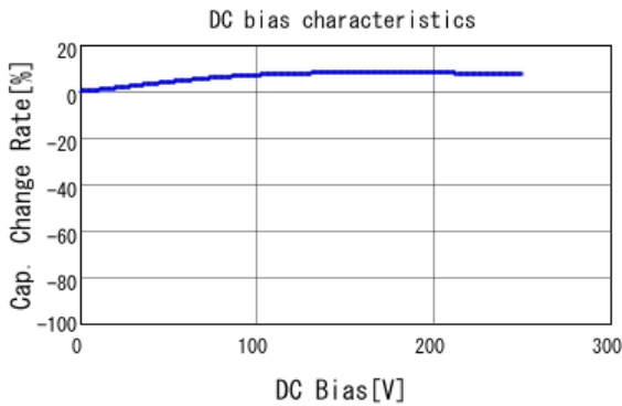
■ DE1E3KX102MA4BN01F C-DC bias capchange, 20.0degC, AC1
