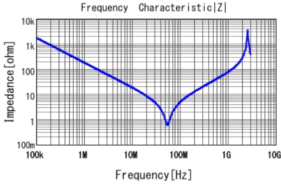
■ DE1E3KX102MA4BN01F |Z| DCOV, 20degC
