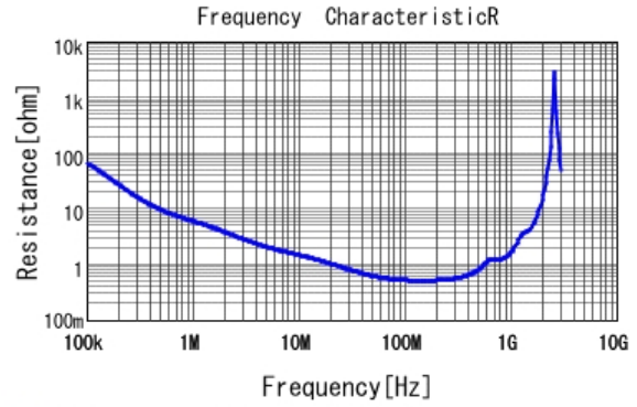
■ DE1E3KX102MA4BN01F R DCOV, 20degC
