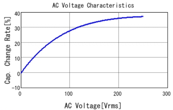
■ DE1E3KX102MA4BN01F C-AC Voltage capchange, DCOV, 20.0
