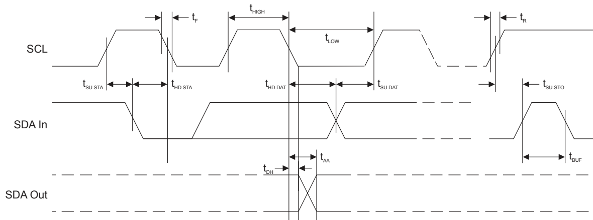
Figure 4-1. Bus Timing
