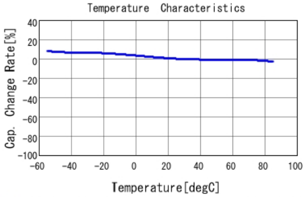
■ GRM155R61E105KA12 C-Temp. capchange, DCO. 0V, AC1. 0Vrm
