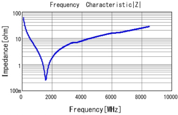
■ GRM1555C1H270JA01 |Z| DCOV, 25degC
