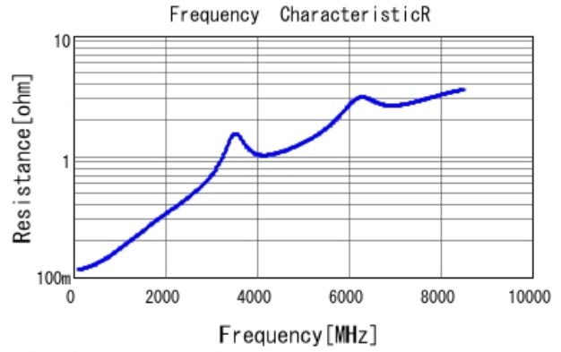
■ GRM1555C1H270JA01 R DCOV, 25degC
