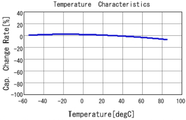
GRM155R61H104KE14 C-Temp. capchange, DC0.0V, AC1.C
