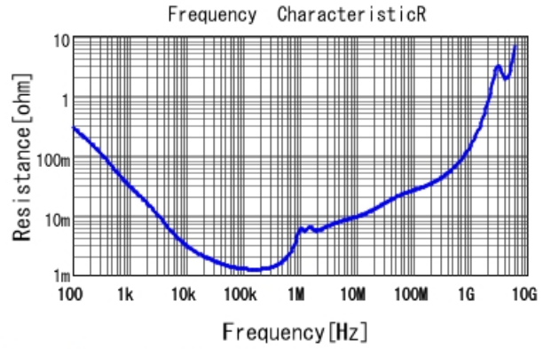
GRM32ER61A107ME20 R DCOV, 25degC
