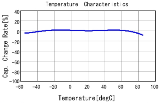
GRM32ER61A107ME20 C-Temp. capchange, DC0.0V, AC0.5
