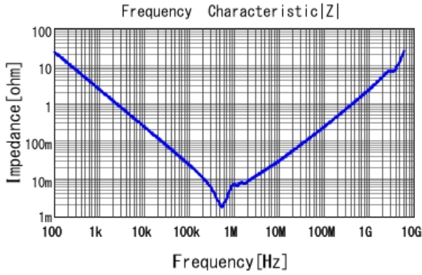
GRM32ER61A107ME20 |Z| DCOV, 25degC
