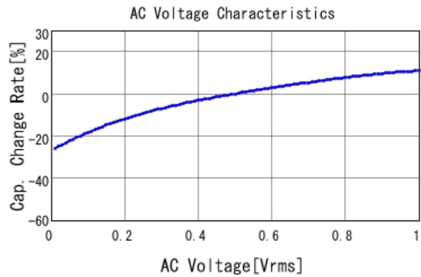
GRM32ER61A107ME20 C-AC Voltage capchange, DCOV, 25
