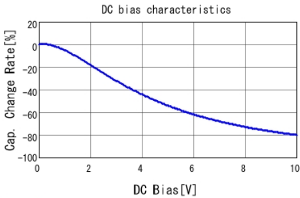
GRM32ER61A107ME20 C-DC bias capchange, 25.0degC, A
