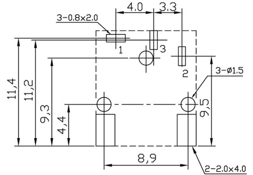
T:1.6 Dimensions of PC board holes Tolerance : \pm 0.05 (Printed-top view)
