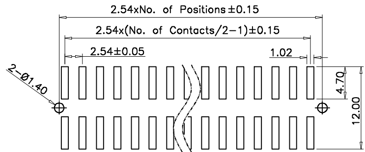
Recommended PCB Layout (PCB TOLERANCE ±0.05)
