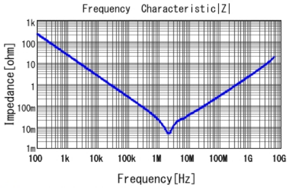
ZRB18AR61E106ME01 |Z| DCOV, 25degC
