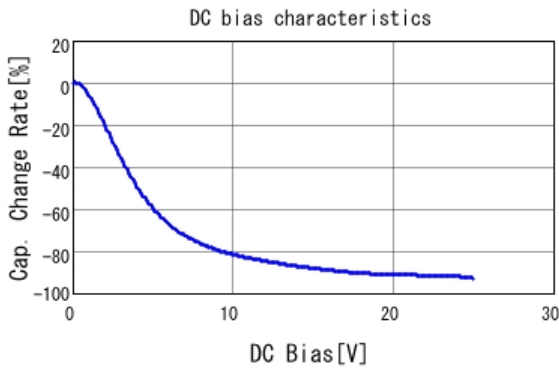
ZRB18AR61E106ME01 C-DC bias capchange, 25.0degC, AC1V
