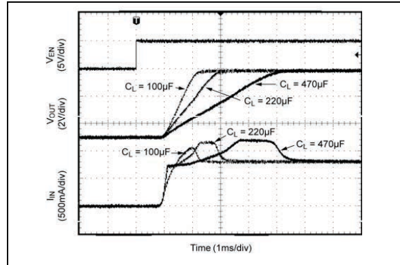
FIGURE 2-40: Current Inrush Current Response.
