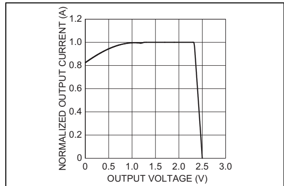
FIGURE 5-4: Normalized Output Current vs. Output Voltage (2.5V).
