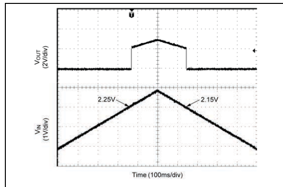
FIGURE 2-30: UVLO.
