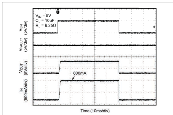
FIGURE 2-27: Enable Turn-On/Turn-Off.
