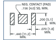
Pad Layout
