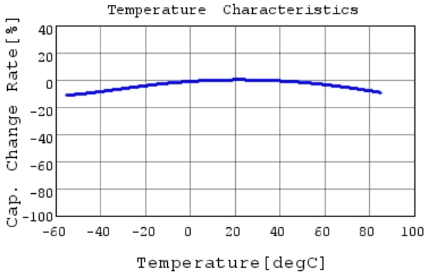
GRM188R61H225KE11 C-Temp. capchange, DC0.0V,
