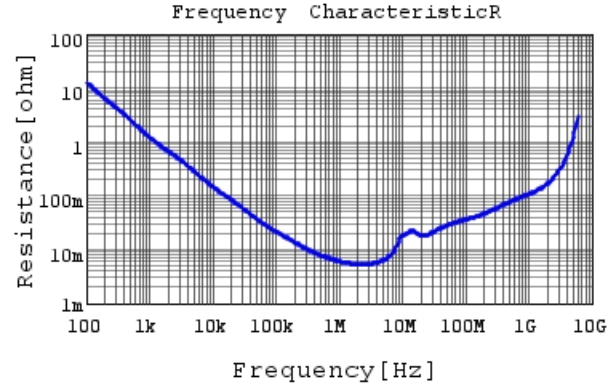
GRM188R61H225KE11 R DCOV, 25degC
