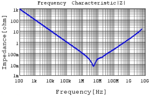
GRM188R61H225KE11 |Z| DCOV, 25degC
