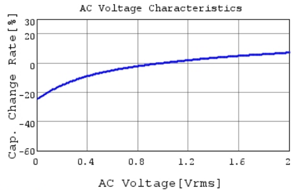
GRM188R61H225KE11 C-AC Voltage capchange, Dc
